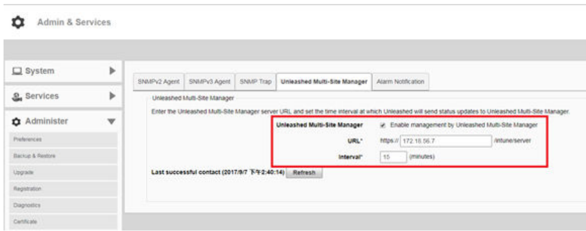
FIGURE 67 Enabling Unleashed Multi-Site Manager Management
