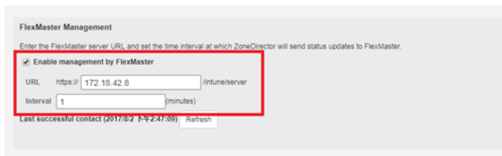
FIGURE 74 Enabling Unleashed Multi-Site Manager Management on ZD
